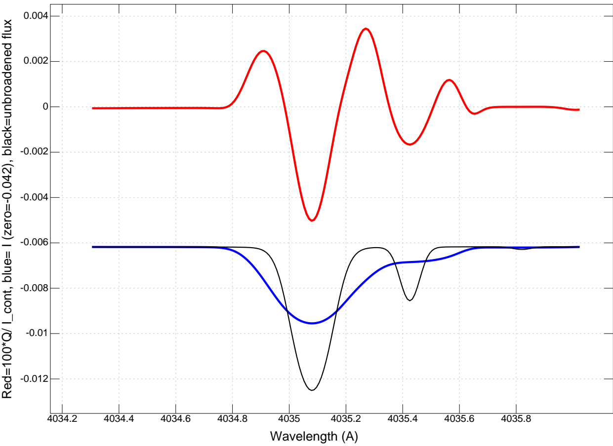
Stokes I&Q across lines of rotating star: T=30,000K, lg=4.0 -- Rot vel = 15 km/s
