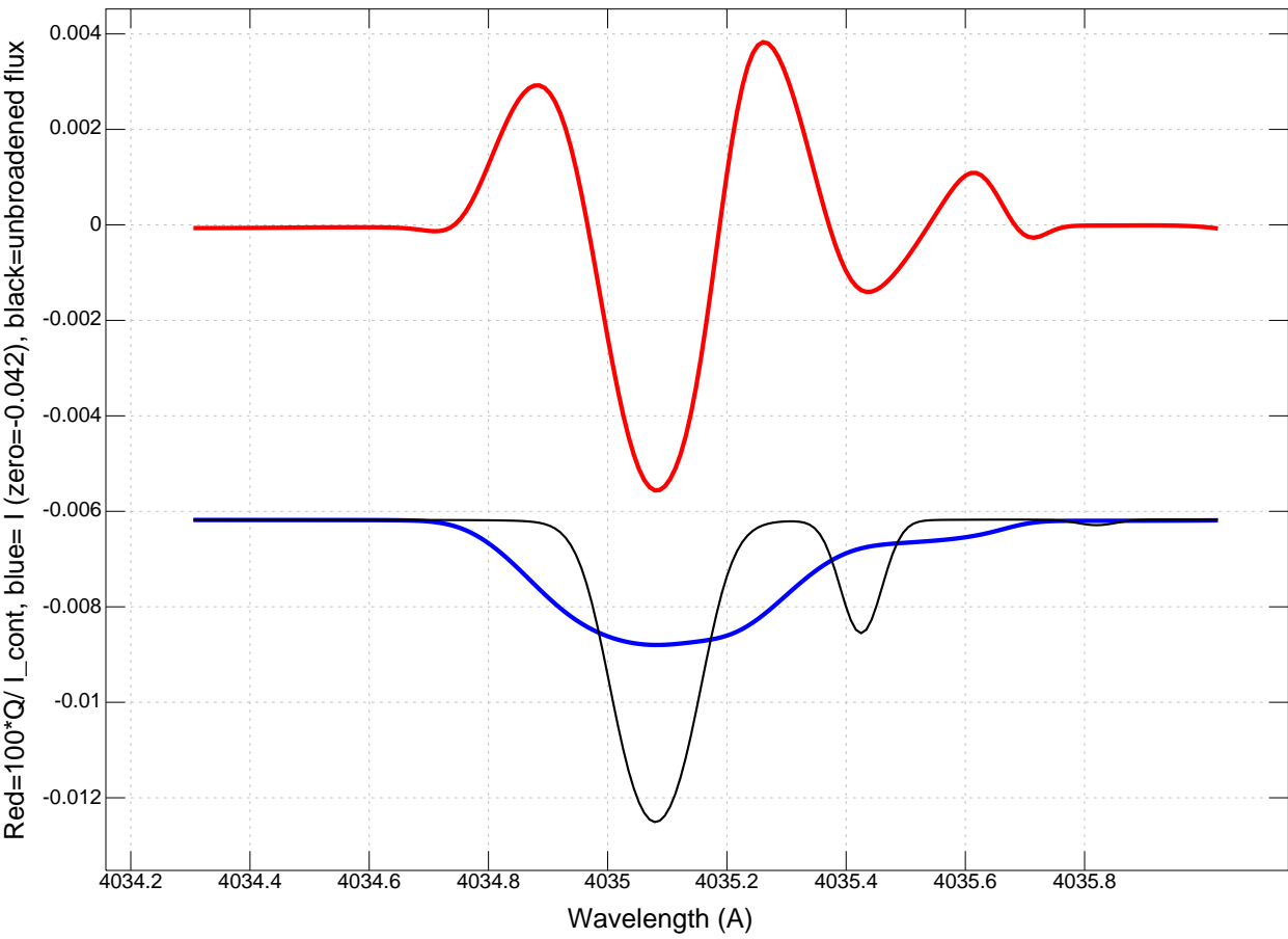
Stokes I&Q across lines of rotating star: T=30,000K, lg=4.0 -- Rot vel = 20 km/s
