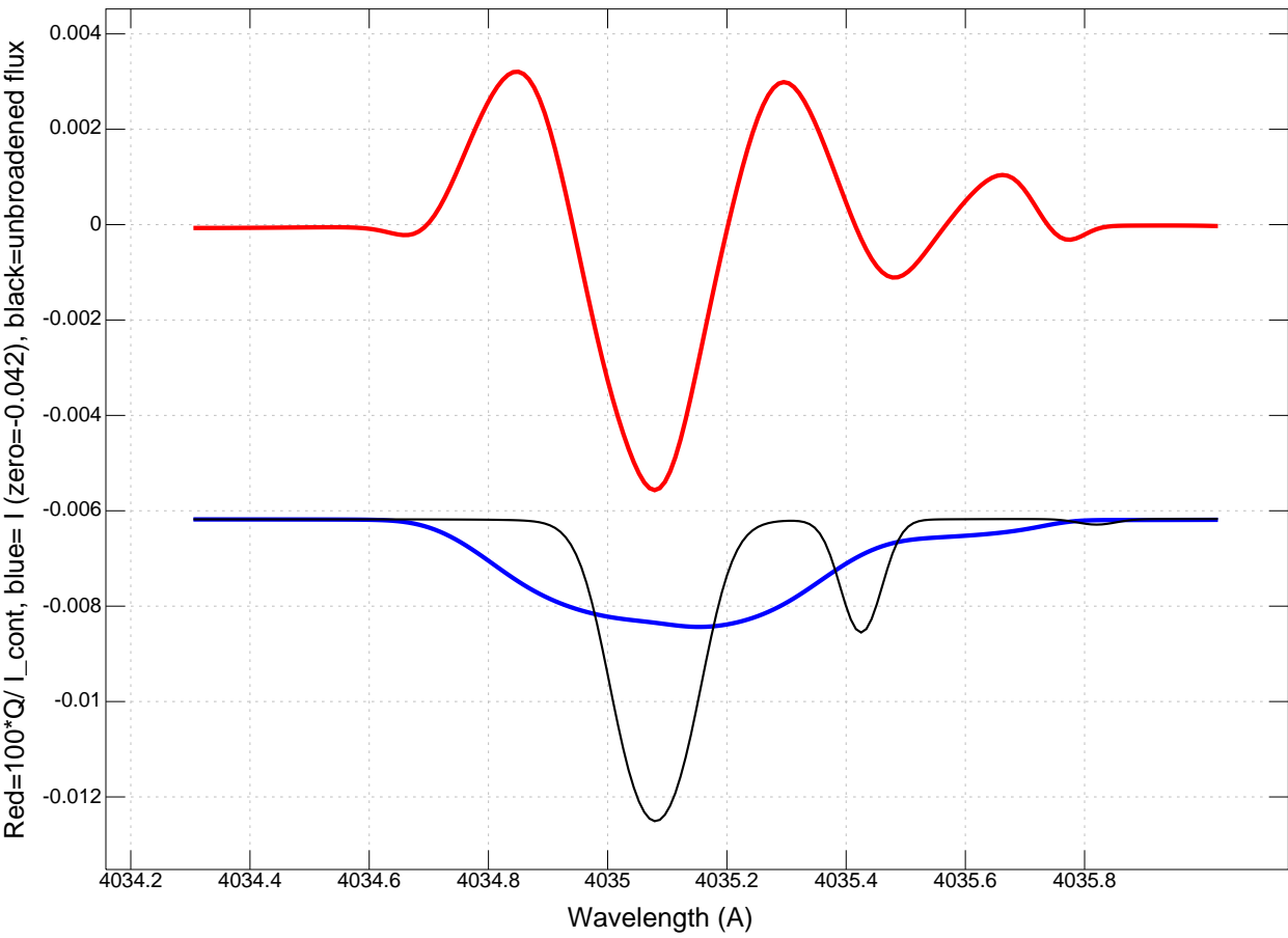
Stokes I&Q across lines of rotating star: T=30,000K, lg=4.0 -- Rot vel = 25 km/s
