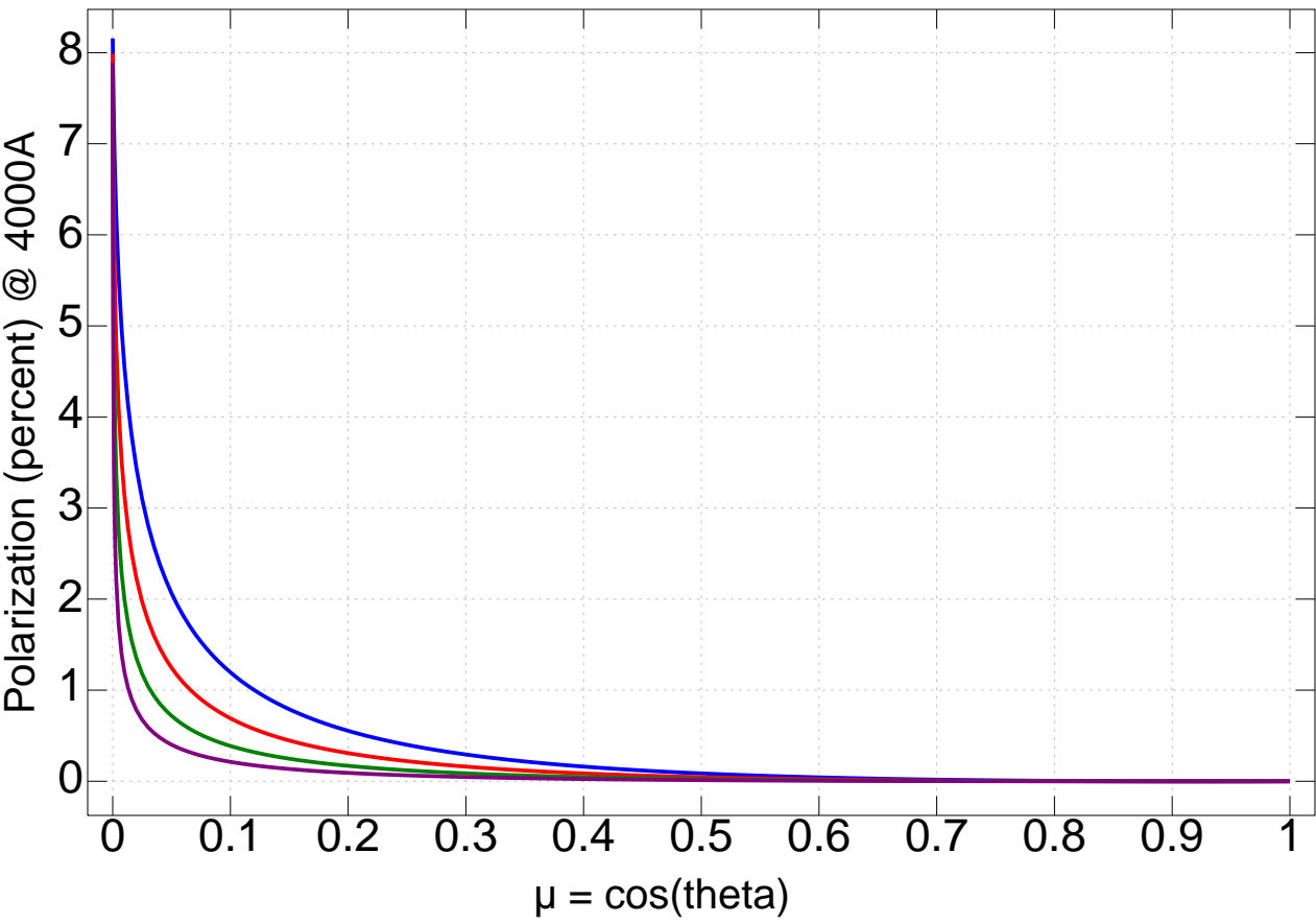
STERNE models: T=12,000K, log g=3.0,3.5,4.0,4.5
