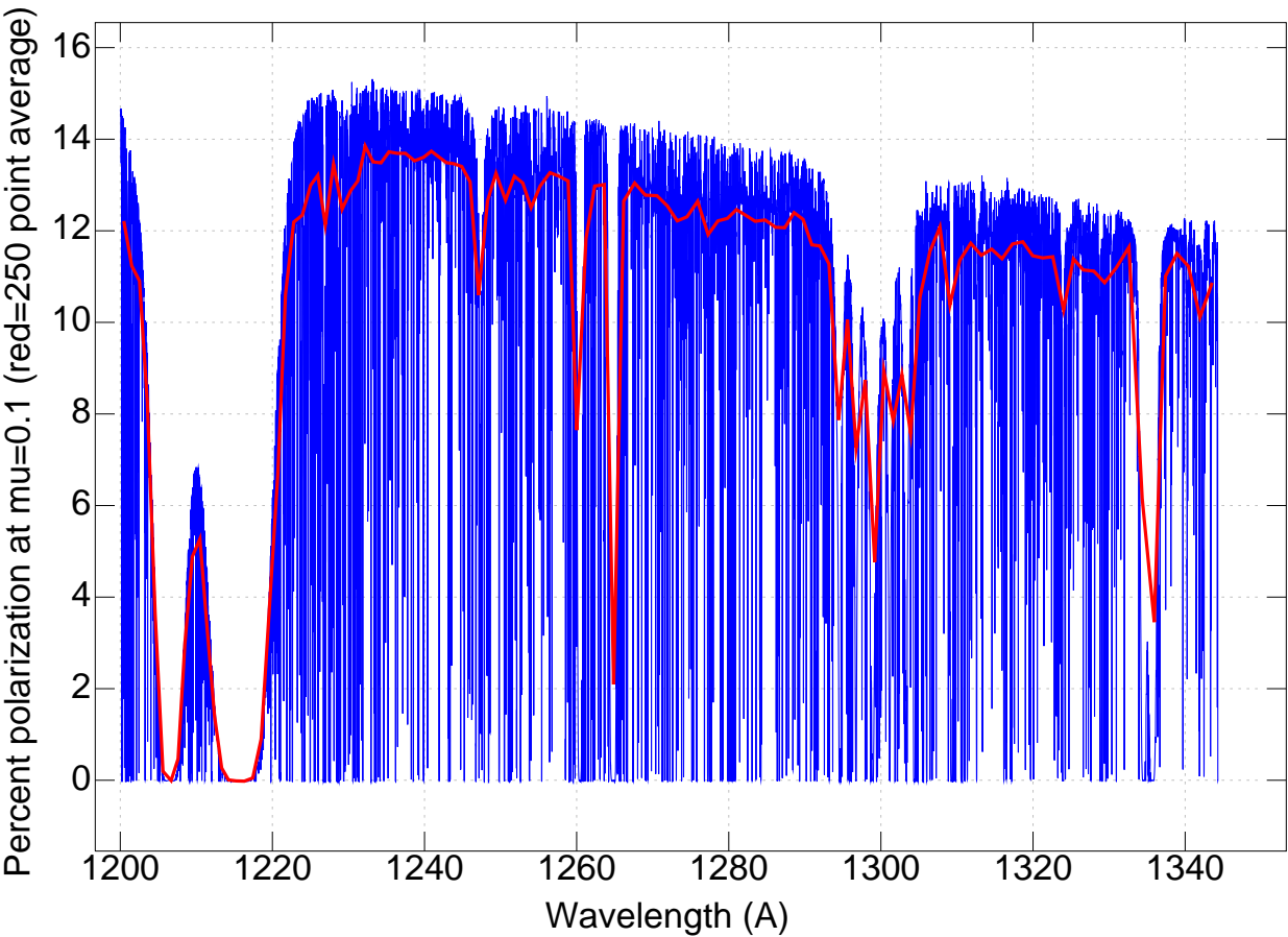
T=15,000, log g=4.5: detailed grid vs average over 250 points
