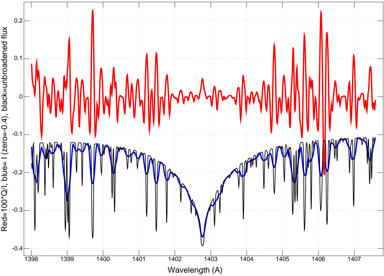
Stokes I&Q across lines of rotating star: T=20,000K, lg=3.5 -- Rot vel = 20 km/s
