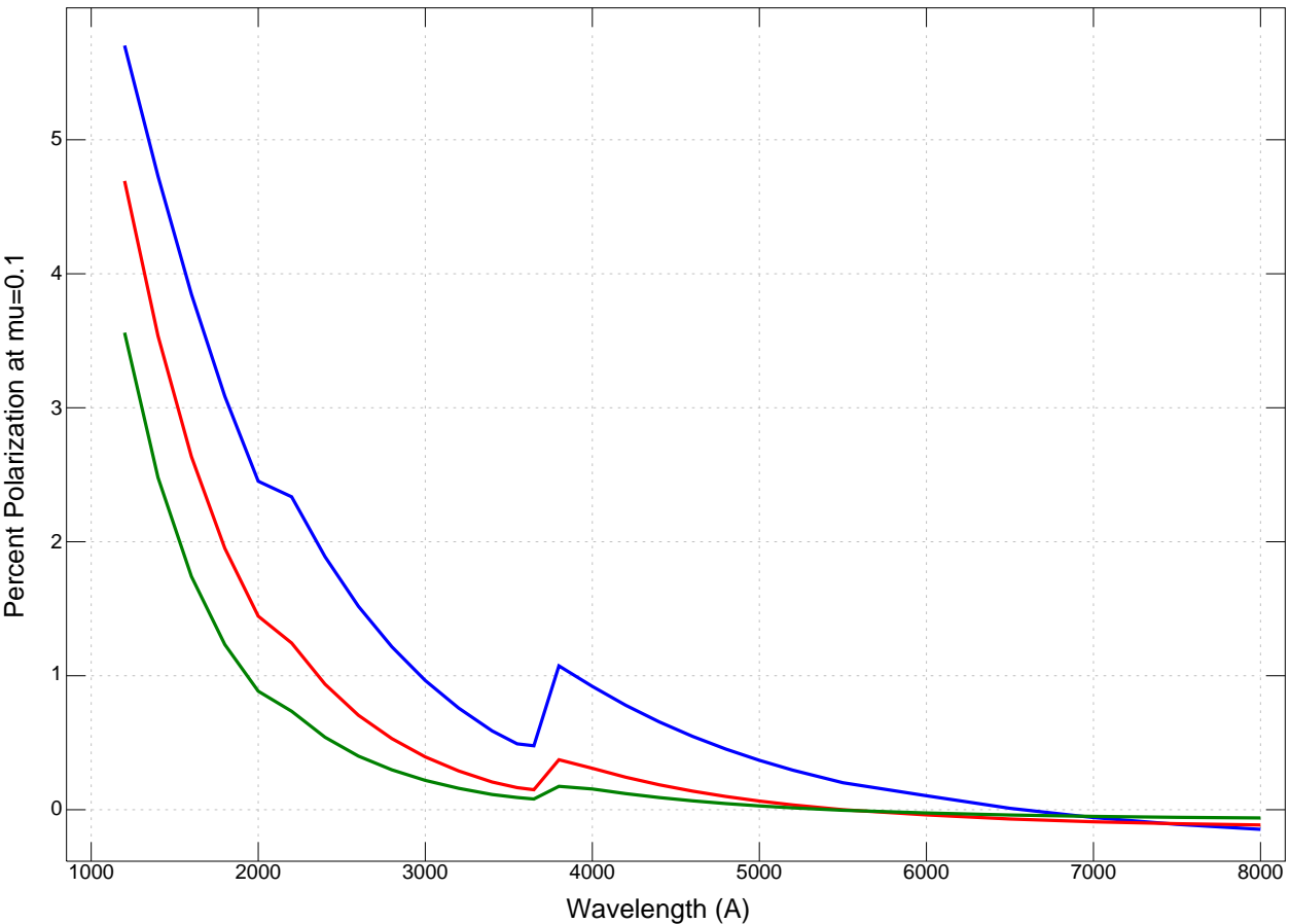
TLUSTY models: T=35,000K log g=3.5,4.0,4.5
