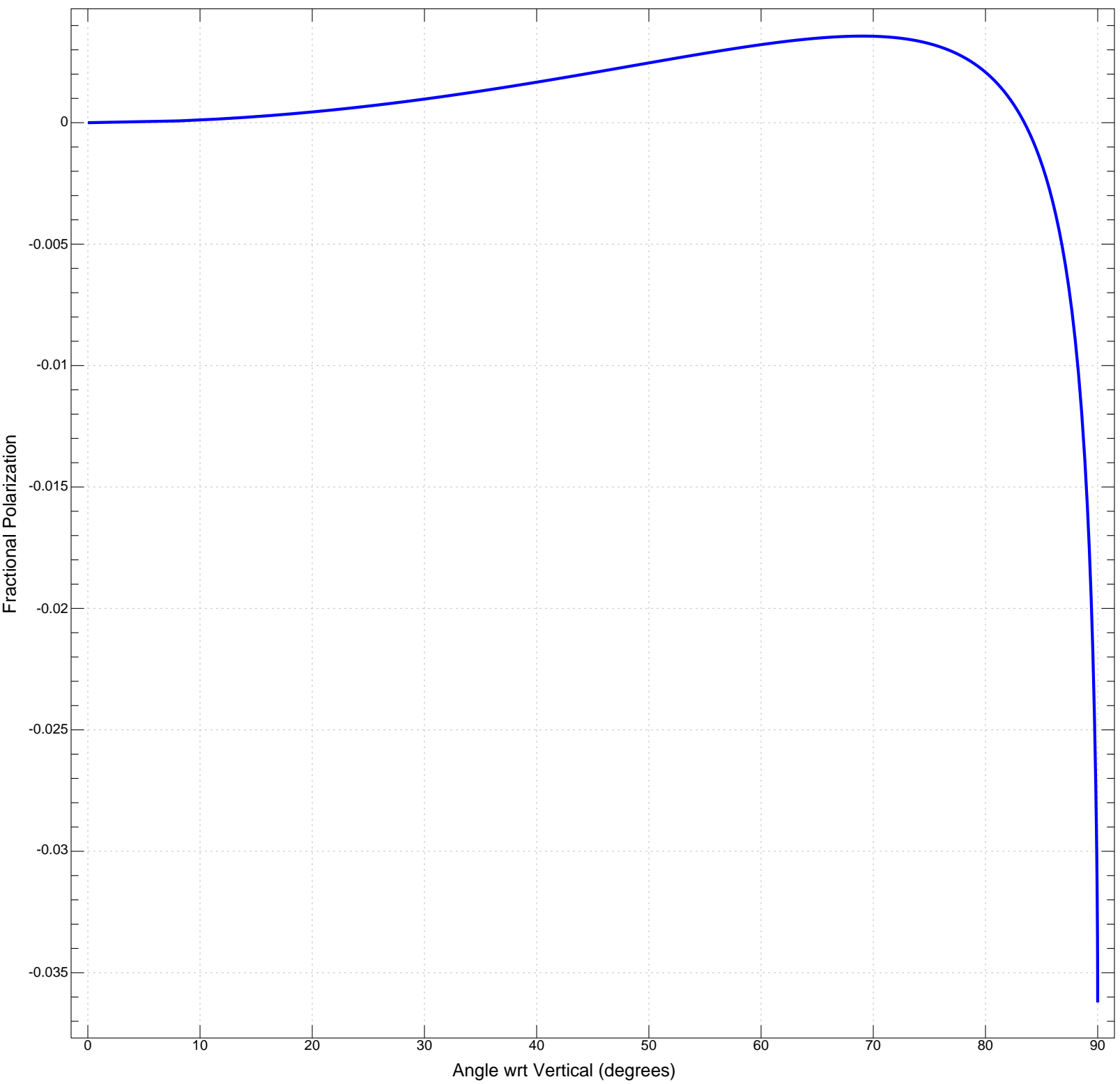
Polarization from Atmosphere with T = 40,000\text{K} & \log(g)=4.0
