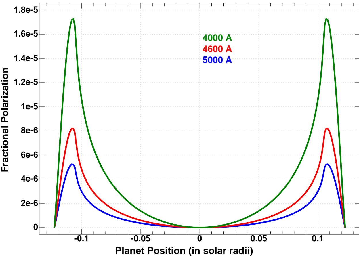
TRAPPIST-1 (T= 2550 K, log g=5.0) center-line transit
