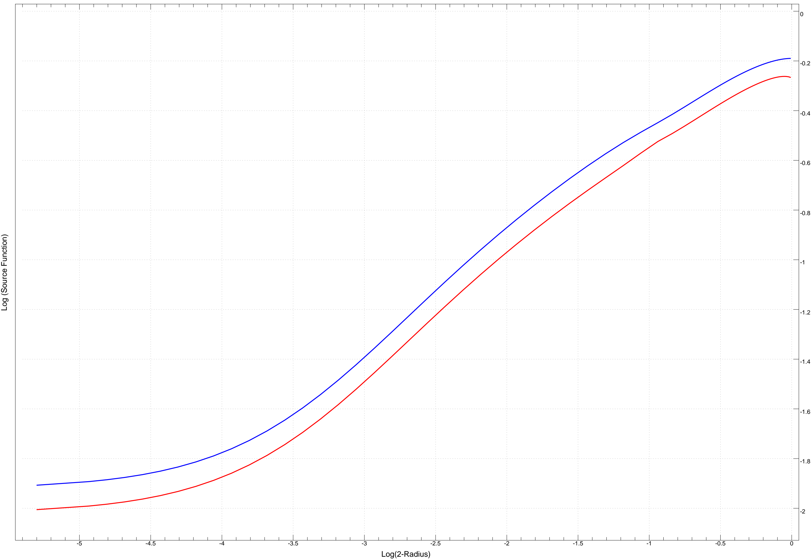
Optical Depth=5000, epsilon=0.0001. Red=sphere, blue=slab.
