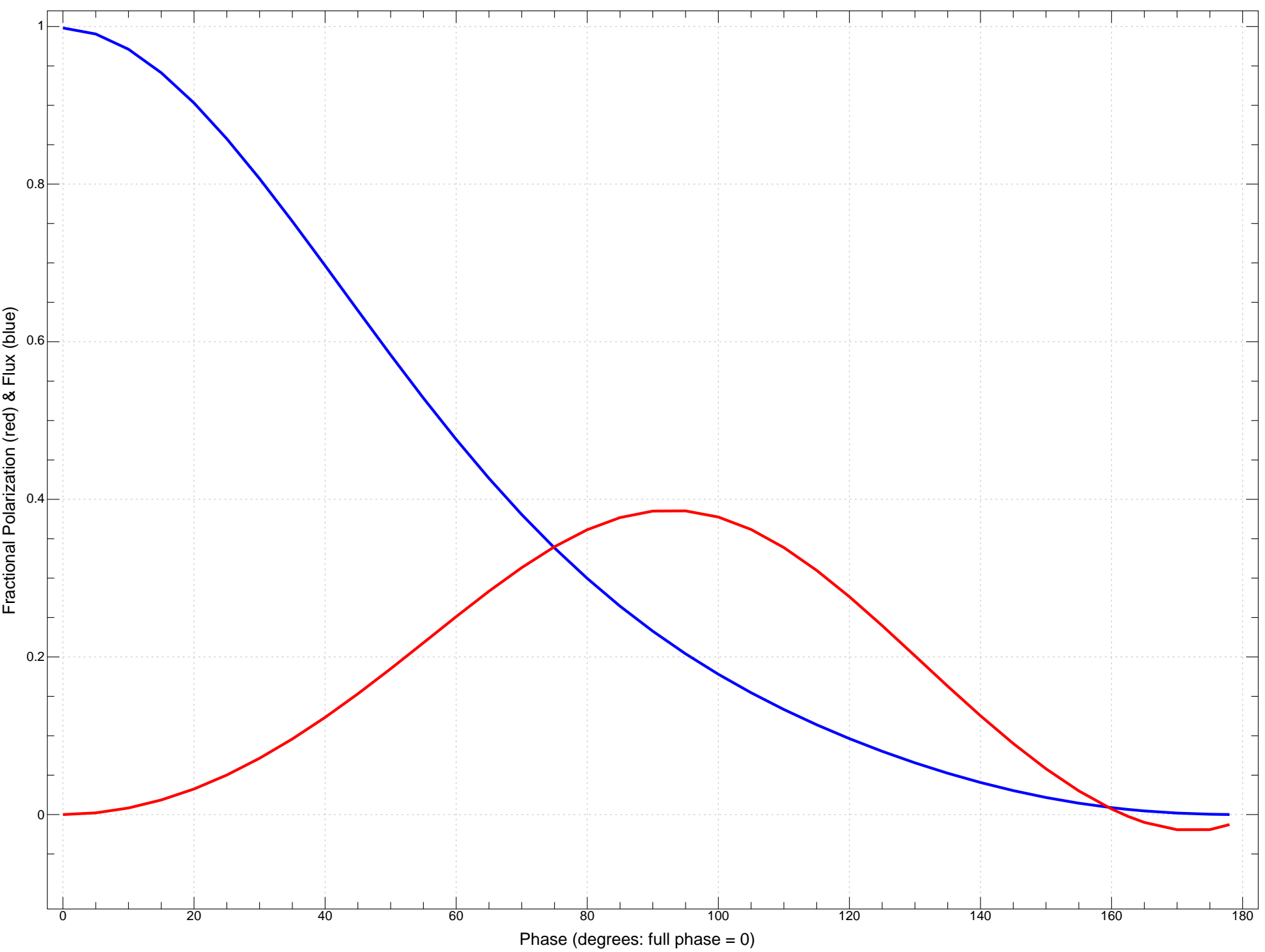
Light Reflected from Planet with Thick Rayleigh-Scattering Atmosphere
