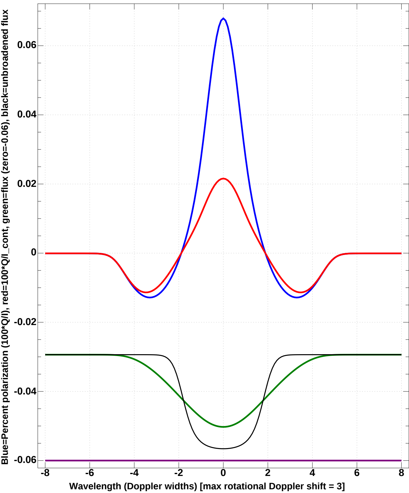
Milne-Eddington \tau(0)=15 line at 4000Å in T=4000\text{K} , \lg=4 , MARCS model
