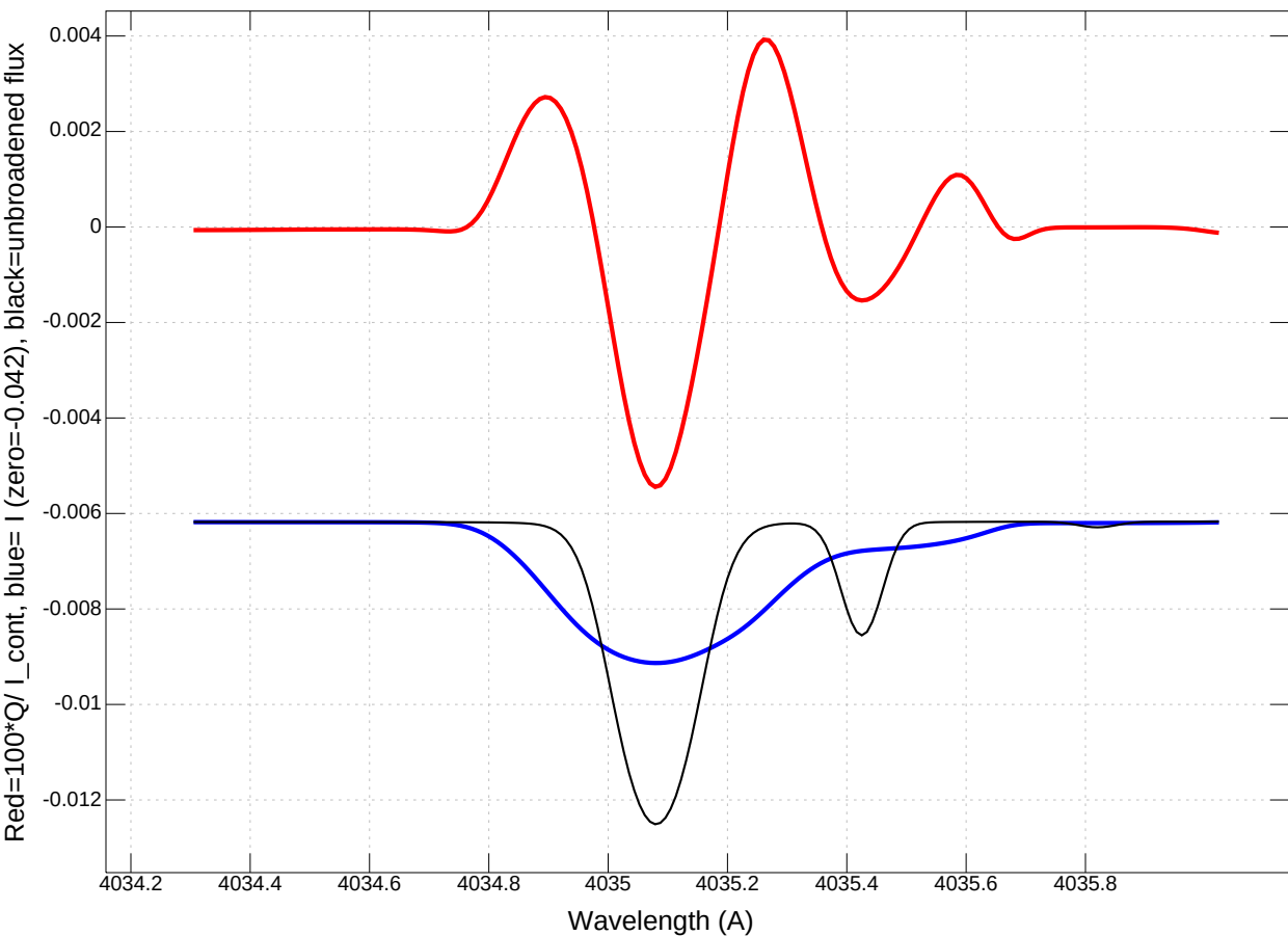
Stokes I&Q across lines of rotating star: T=30,000K, lg=4.0 -- Rot vel = 17.5 km/s
