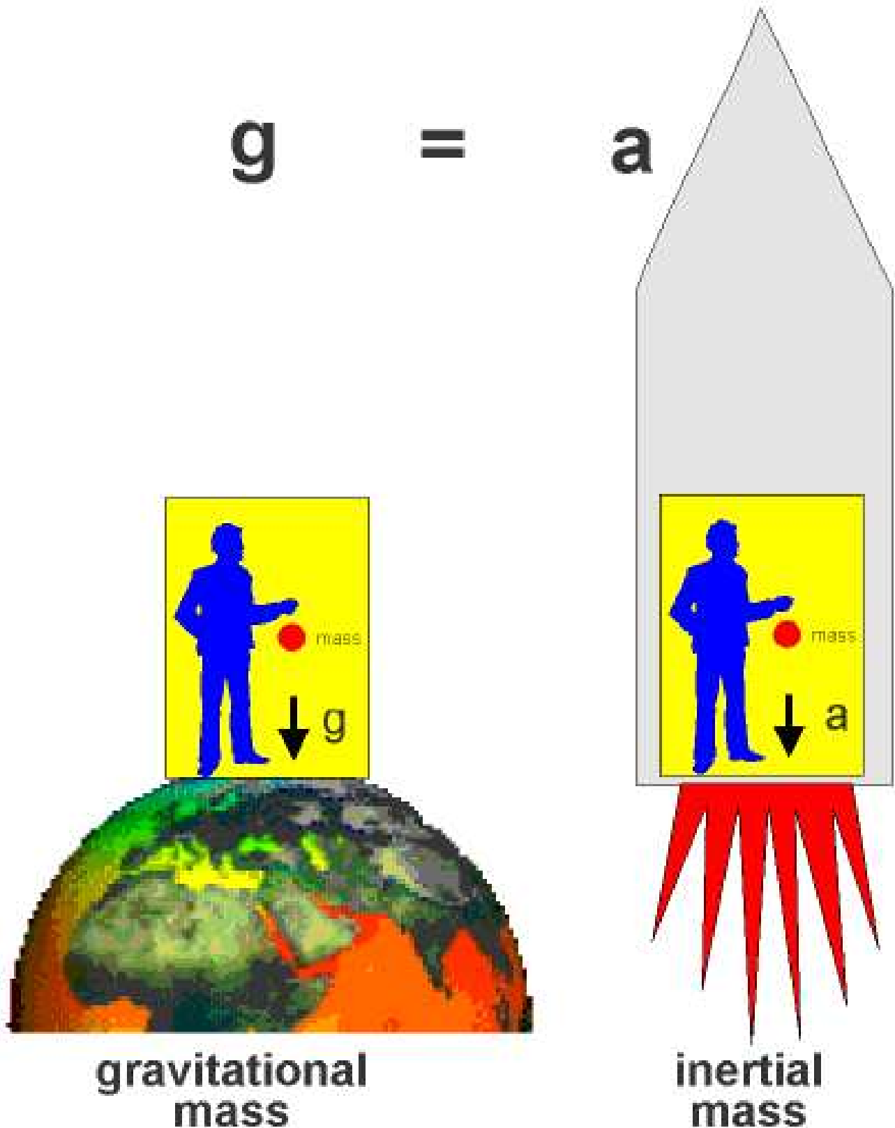
Fig. 1.— One facet of the equivalence principle: locally, gravity looks like accelerated flat spacetime. From http://www.desc.med.vu.nl/Graphics/Equiv_principle.gif
