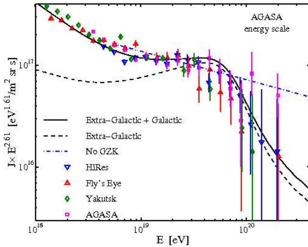
Fig. 1.— Some recent data on high-energy cosmic rays, from several experiments. From http://www.astro.psu.edu/users/nnp/fig_agasa_norm.gif
