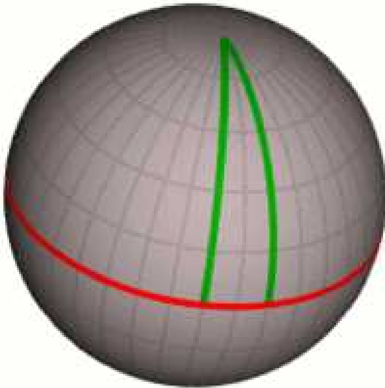
Fig. 1.— Because a sphere's surface is curved, nearby geodesics deviate from each other. From http://upload.wikimedia.org/wikipedia/commons/thumb/2/24/Earth_geo.gif/250px-Earth_geo.gif
