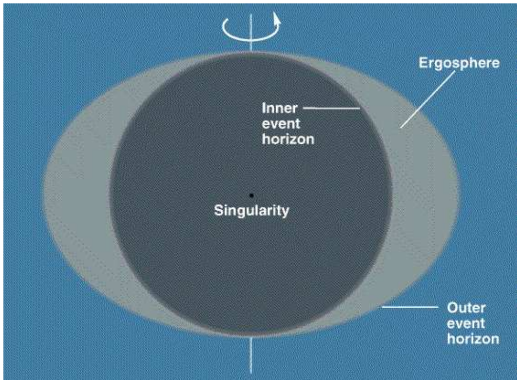
Fig. 1.— Features of a rotating (Kerr) black hole. It has a horizon and a singularity, just like a nonrotating (Schwarzschild) black hole. However, it also has a region outside the horizon called the ergosphere, in which as seen at infinity everything must rotate in the same direction as the hole. From http://www.zamandayolculuk.com/cetinbal/KO/KerrBlackHoleFeatu.gif
