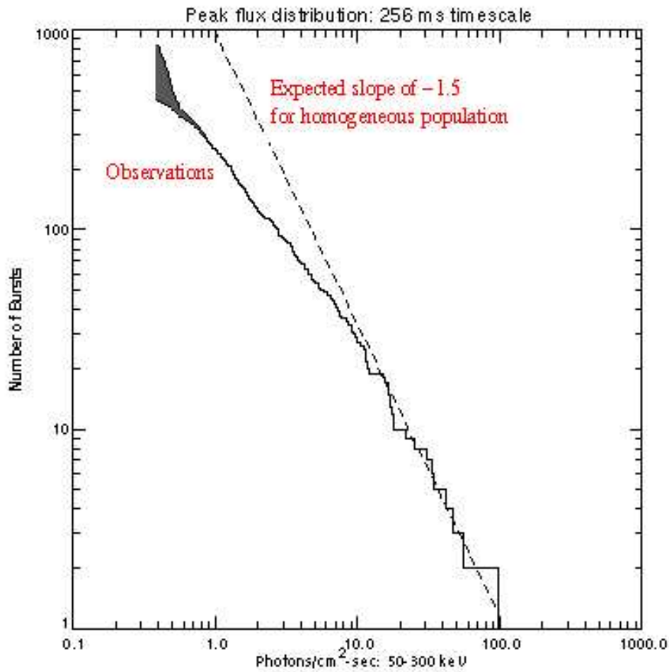
Fig. 1.— Cumulative log number vs. log flux diagram for gamma-ray bursts detected with the BATSE instrument. The straight line is what would be expected if the sources were distributed homogeneously in a Euclidean universe. The rollover at low fluxes is one indicator of a cosmological population. From http://aether.lbl.gov/www/projects/neutrino/grb/logn_logs.gif
