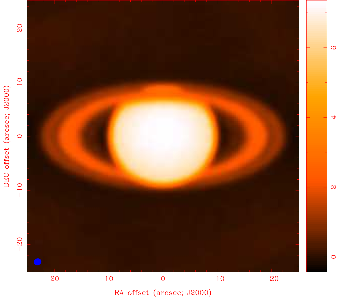
Fig. 5.— Joint deconvolution image using CARMA CZ + DZ configurations including all the cross correlations between the CARMA and SZA arrays, but omitting the short spacings between 3.5 and 6.1 m which are sampled by the compact SZA array. Gaussian beam FWHM 1.41 x 1.26 arcsec, shown in lower left corner.
