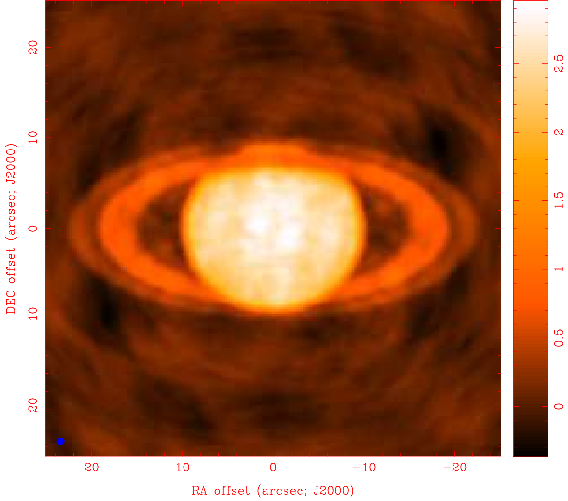
Fig. 2.— Joint deconvolution image using the CARMA CZ configuration, including all the cross correlations between the CARMA and SZA arrays, but omitting the short spacings between 3.5 and 6.1 m which are sampled by the compact SZA array. Gaussian beam FWHM 0.87 x 0.76 arcsec, shown in lower left corner
