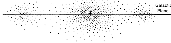
FIG. 3—Arthur Eddington's (1912) galaxy placed the Sun's position 60 LY above the center of the galactic plane.
