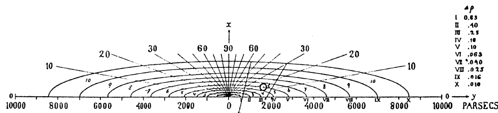
FIG. 4—Kapteyn and van Rhijn (1920) and Kapteyn (1922) deduced galactic dimensions based on star counts with no allowance for absorption by dust.
