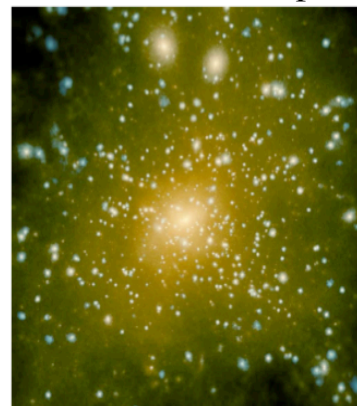
Dark matter simulation V.Springel
