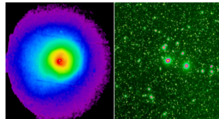
X-ray optical Perseus cluster d~73 Mpc
