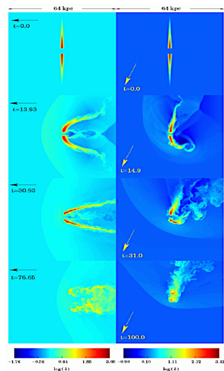
Quilis, Moore, & Bower 2000: Ram pressure induced gas stripping; 18 Timescale ~100 Myr
