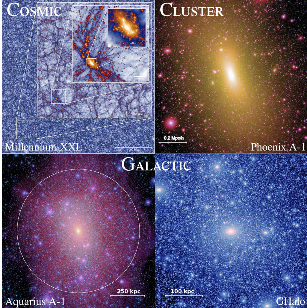
Figure 3: Visualizations of state of the art simulations on cosmic (Millennium-XXL [205], upper left), cluster (Phoenix A-1 [248], upper right), and galactic scale (Aquarius A-1 [39], lower left, and GHalo [27], lower right).
