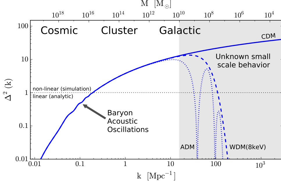
Figure 1: \Delta^2(k) \equiv 4\pi(k/2\pi)^3 P(k) , the linear power spectrum of density fluctuations at z = 0 . The solid line is the canonical cold DM model with an Eisenstein & Hu (1997) [10] transfer function. The dashed line is a thermal relic warm DM model with m_{\text{WDM}} = 8 \text{ keV} [11]. The dotted line is an atomic DM model [12]. We used WMAP7 cosmological parameters [13], \Omega_m = 0.265 , \Omega_\Lambda = 0.735 , \Omega_b = 0.0449 , h = 0.71 , \sigma_8 = 0.801 , and n_s = 0.963 .
