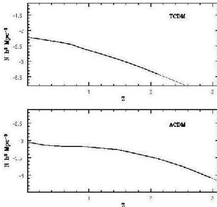
Figure 3: The abundance of massive ( >10^{11}M_{\odot} ) systems as a function of redshift in two hierarchical models (Kauffmann & Charlot 1998) showing the strong decline in a high density ( \tau CDM) model c.f. that in a low density accelerating model ( \Lambda CDM).
