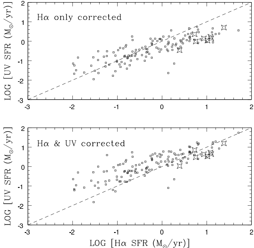
Figure 5: Star formation rates derived from UV (2000 Å) continua versus those derived from H \alpha fluxes from the local survey of Sullivan et al (2000, open squares) and the z \simeq 1 samples of Glazebrook et al (1999, large stars). For the Sullivan et al sample, extinction corrections were derived from individual Balmer decrements assuming Case B recombination and applied to the H \alpha fluxes in the upper panel and both estimates in the lower panel.
