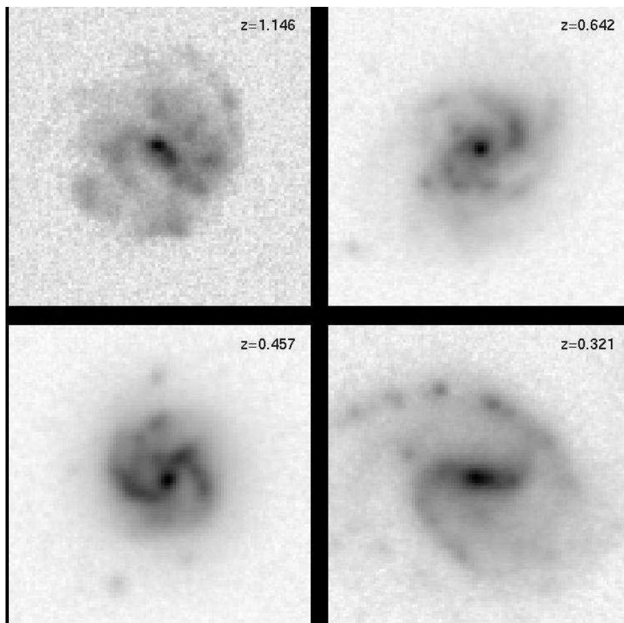
Figure 18: Face-on barred spirals of known redshift in the Hubble Deep Field. Abraham et al (1999) claim that all such systems should easily be recognised to z \approx 1 in HDF-quality data whereas, beyond z \approx 0.6 , there appears to be a marginal paucity of such systems compared to their non-barred counterparts. If supported by further data, this could indicate an epoch corresponding to the ‘dynamical maturing’ of stellar disks.
