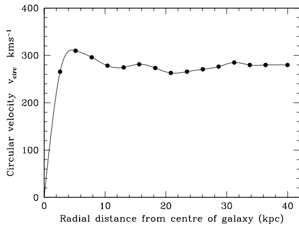
Figure 5.1: The spiral galaxy NGC 2841 and its HI 21 cm radio rotation curve. The figure on the left presents an optical (blue light) image of the galaxy, while that on the right gives the rotation curve in the form of the circular velocity plotted against radial distance. The optical image covers the same area of the galaxy as the radio observations: the 21 cm radio emission from the atomic hydrogen gas is detected over a much larger area than the galaxy covers in the optical image. [The optical image was created using Digitized Sky Survey II blue data from the Palomar Observatory Sky Survey. The rotation curve was plotted using data by A. Bosma (Astron. J., 86, 1791, 1981) taken from S. M. Kent (AJ, 93, 816, 1987).]
