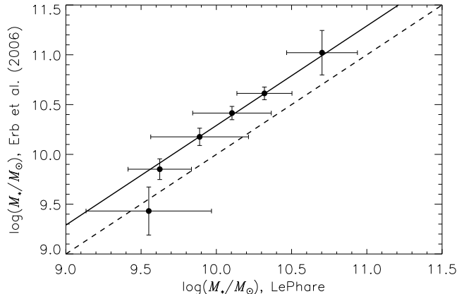
FIG. 1.— The stellar mass determined by Erb et al. (2006c) plotted against our determination using LePhare. The dashed line is the one-to-one agreement and the solid line is offset by 0.29 dex. In the five higher mass bins, the stellar mass estimates used in E06 are greater by a factor of 2 (0.29 dex).
