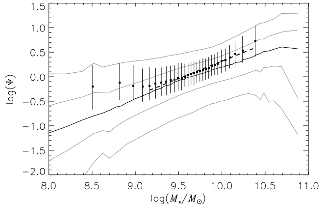
FIG. 5.— The SFR ( M_{\odot} \text{ yr}^{-1} ) plotted against stellar mass for our metallicity selected SDSS sample (black points) along with larger comparison sample from SDSS. The black points and error bars are the observed MS relation and its scatter for our metallicity selected SDSS sample. The dashed black line is our fitted relation given by Equation 8 with parameters given in Table 2. The solid black curve is the MS relation for our larger comparison sample and the gray lines are the 68 and 95% contours.
