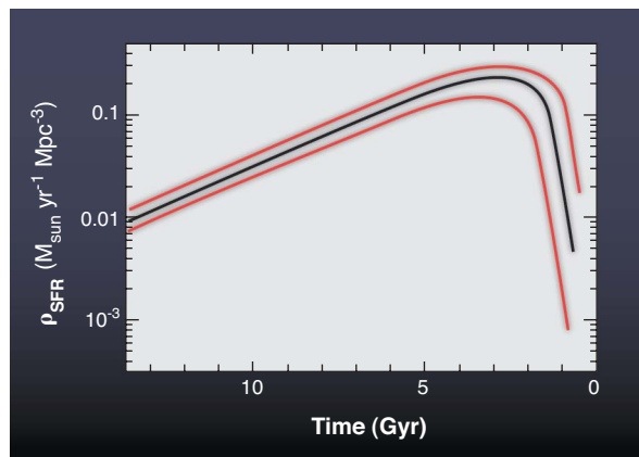
Fig. 2. A simple representation of our current knowledge of the rise and fall of globally averaged star-formation activity over the 13.7 billion years of cosmic history. The black line indicates our best estimate of how the density of star formation (in solar masses formed per year per unit of co-moving volume) grew rapidly in the first 2 billion years after the Big Bang, stayed roughly constant for a further \sim 2.5 billion years, then has declined almost linearly with time since the universe was \sim 5 billion years old. The red lines indicate the typical current uncertainty in the measurement, which rises to approximately an order of magnitude at the earliest times.
