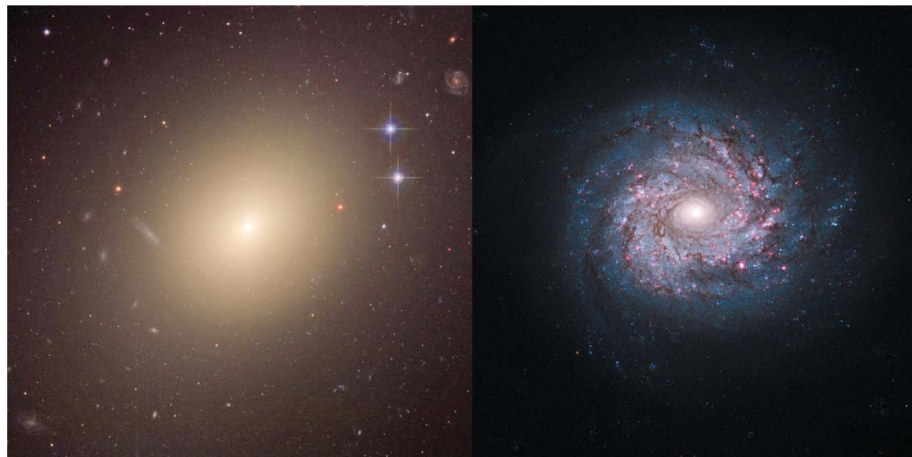
Fig. 1. As shown by the Hubble Space Telescope image of the elliptical galaxy ESO 325-G004 (left), massive galaxies in the nearby universe are overwhelmingly dominated by old red/yellow stars formed more than 10 billion years ago and show little evidence of recent star-formation activity. By contrast, lower-mass galaxies generally continue to form stars in the present day, as shown by the young blue star clusters, red clumps of ionized hydrogen gas, and dark regions of cool dust and gas shown in the Hubble Space Telescope image of the spiral galaxy NGC 3982 (right).
