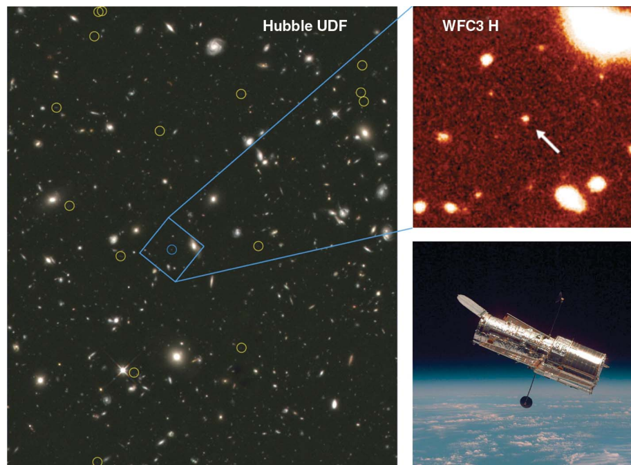
Fig. 3. The deepest ever near-infrared image of the sky, taken with the new WFC3 on board the refurbished Hubble Space Telescope (lower right). This image, shown at left, is in a small region of sky called the Hubble Ultra Deep Field (HUDF) and has led to the discovery of the first galaxies at redshift z = 7 to 8 (indicated by yellow circles). The upper-right panel shows a zoom in to the 1.6- \mu\text{m} image of one of these galaxies, at redshift z = 7.2 , seen when the universe was only 750 million years old.
