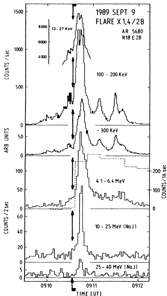
FIG. 1.—The 1989 September 9 flare as seen in X-rays and \gamma -rays by SMM (Rieger 1991). A short pulse of high-energy emission is observed roughly 50 s after the onset in hard X-rays. It consists of electron bremsstrahlung up to 40 MeV and nuclear line emission between 1 and 7 MeV. The dashed line denotes the intensity of the 2.2 MeV neutron capture line (right-hand scale). The arrows and the thick bars mark onset and duration of the spatially and spectrally isolated radio source at 327 MHz reported by Chupp et al. (1993); see the discussion in § 3.
