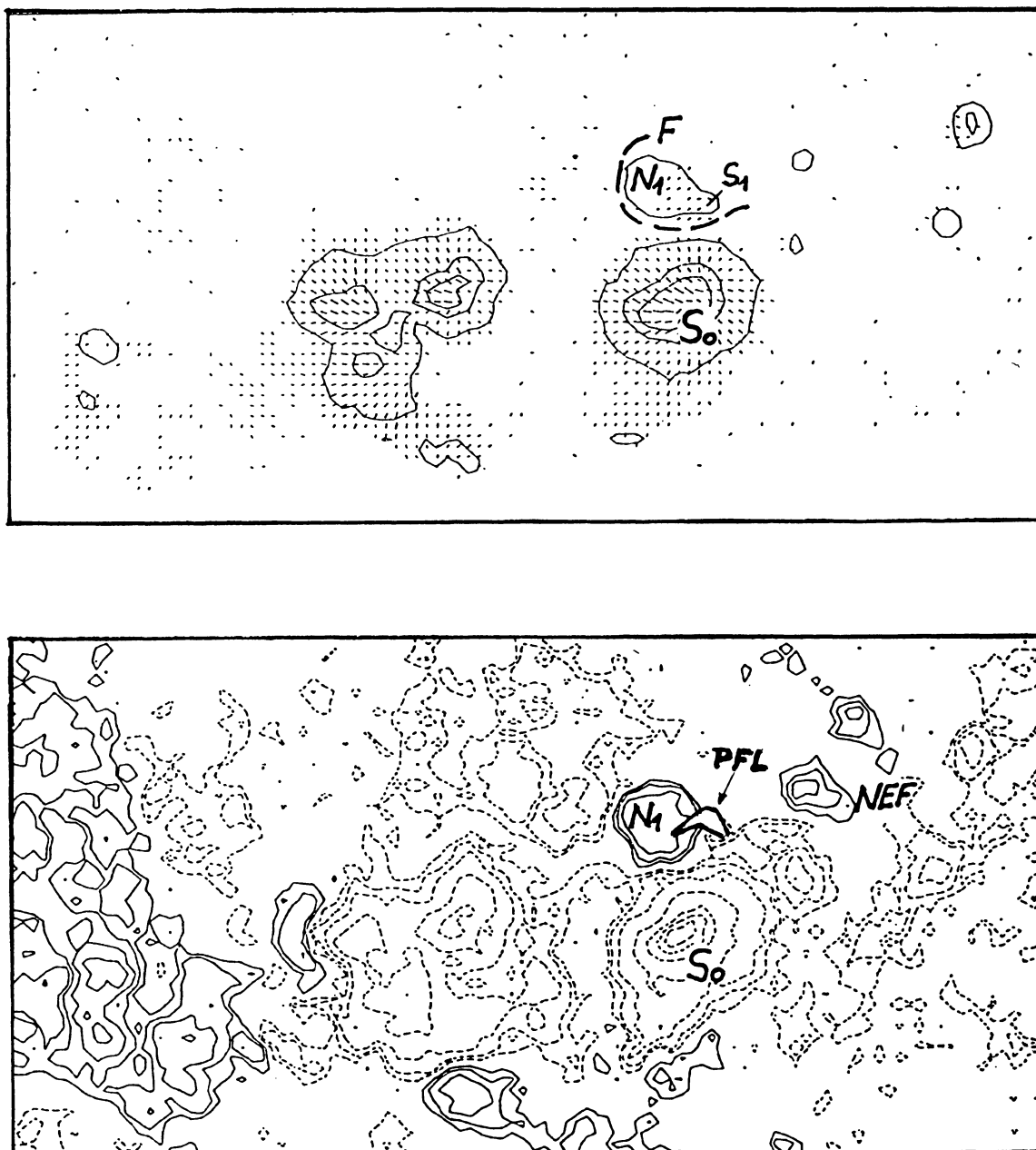
FIG. 2.—The Potsdam magnetogram ( 5250.2 \text{ \AA} blue wing) of 1989 September 9 taken between 07:37 and 08:44 UT. The upper-left-hand corner of the picture ( 276' \times 138'' ) is at N24 E41; north is top, east is left. Top : brightness contours and azimuth of the transversal field component. Isoline levels (quiet Sun = 1000): 850, 550, 300. S_0 : the large leading south polarity spot; N_1 : nearly circular north polarity structure being the follower of the small-scale bipolar region ( S_1 , N_1 ) which in white light is a pore accompanied by a nonregularly stretched penumbra; F : a nearly circular active region filament. Bottom : the corresponding longitudinal field magnetogram. Isoline levels 40, 80, 160, . . . , 1280. Solid : north; dashed : south. PFL : postflare loops from an earlier flare, visible on a Potsdam H\alpha image; NEF : region of newly emerging north polarity magnetic flux. A south polarity NEF region is positioned about 81,000 km to the northwest and was out of the actual field of view of the magnetograph.
